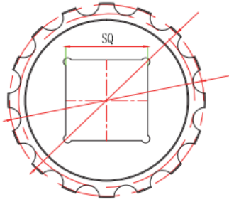
Square bore
