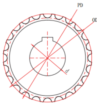
Round bore with keyway
