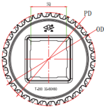
Square bore
