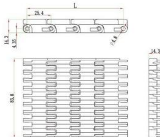
parts P306-332
